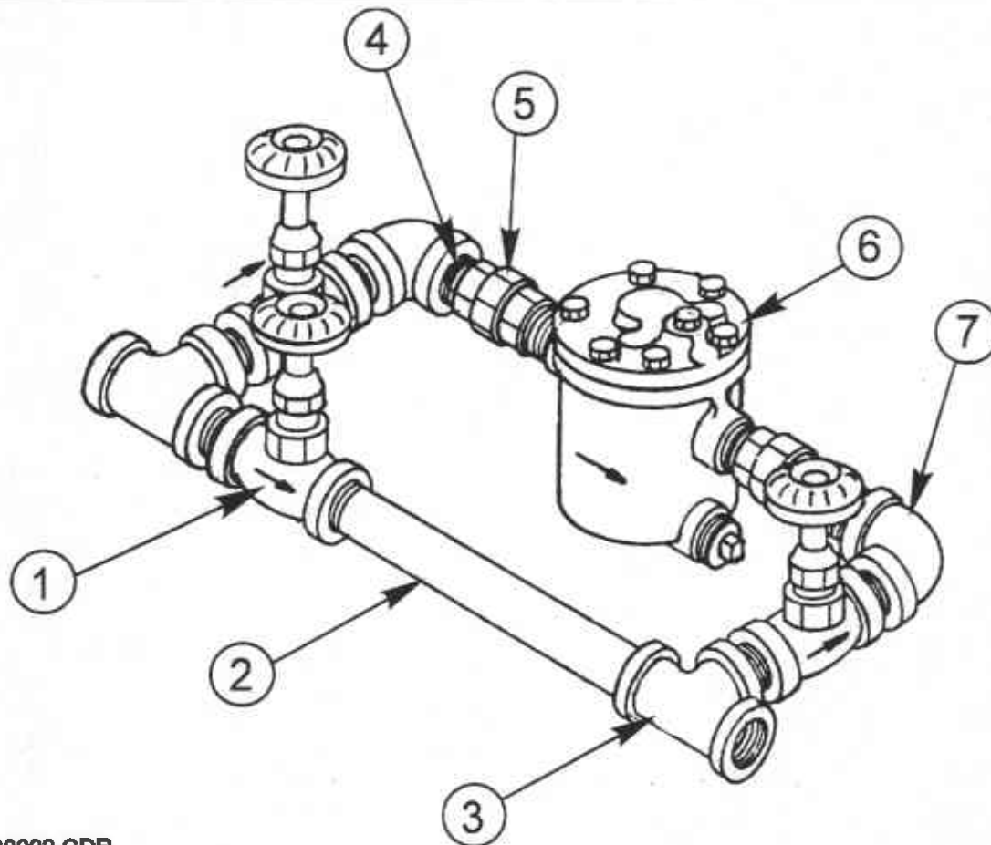
Figure 6-20. By-Pass & Trap Option
