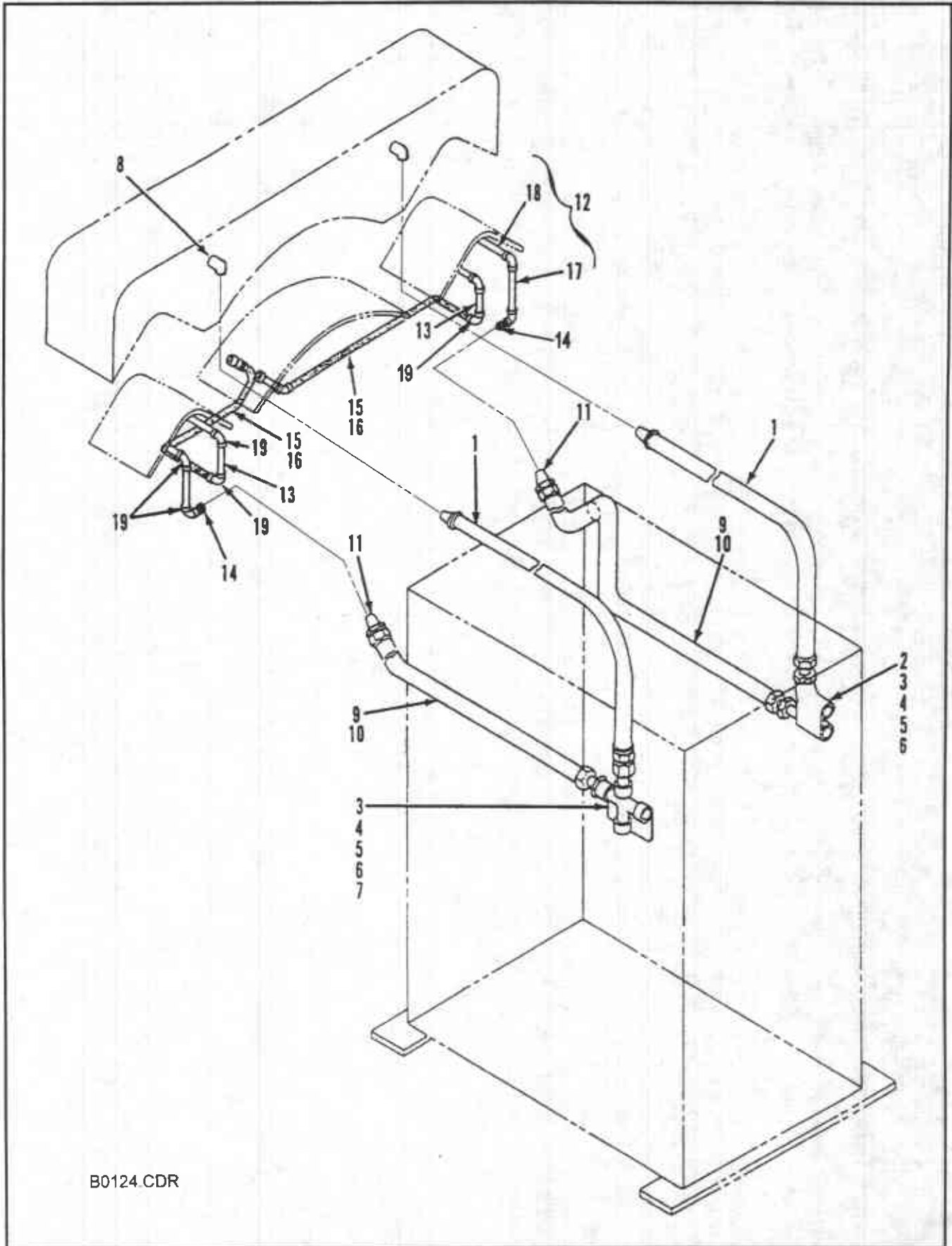
Figure 6-15. Steam System
