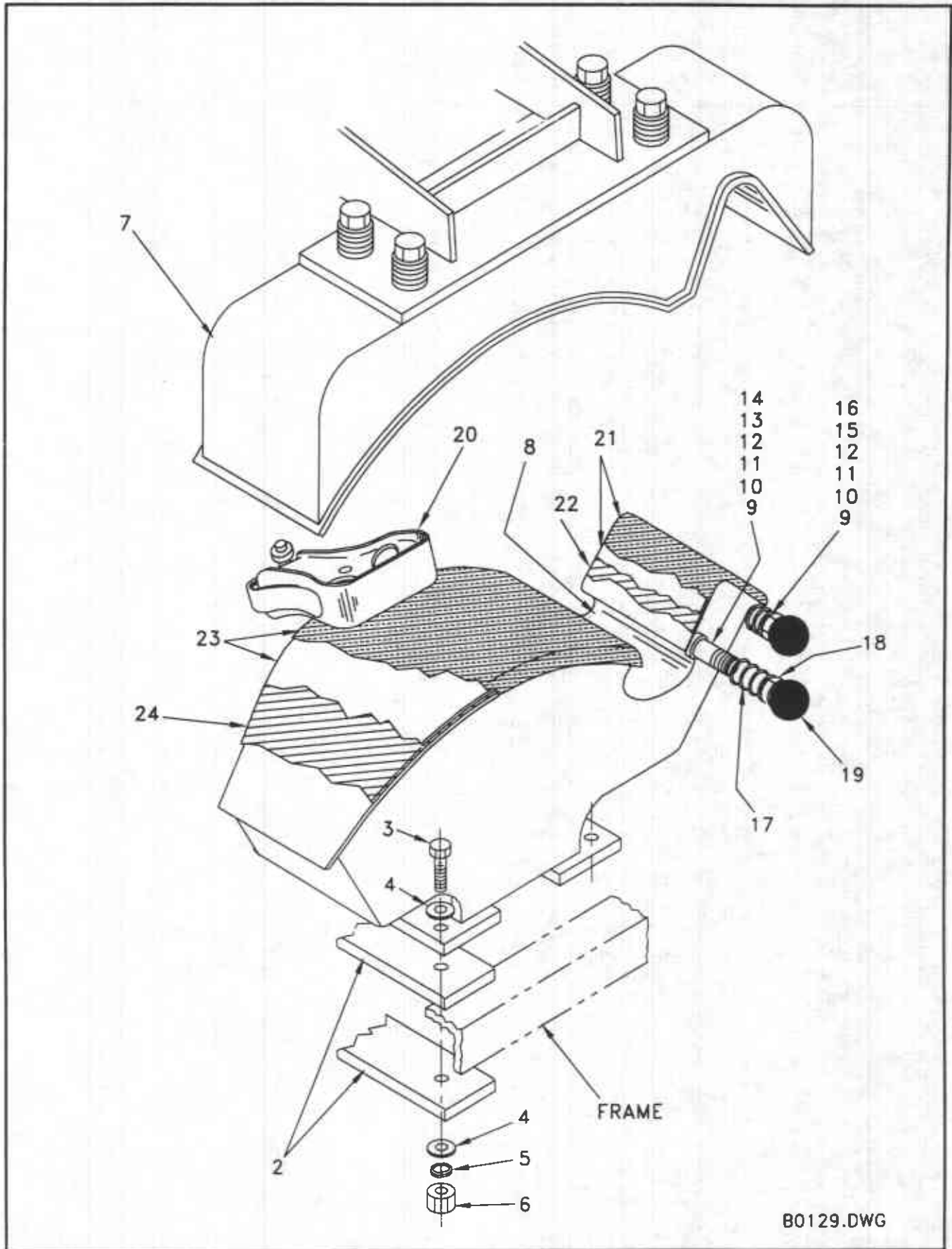
Figure 6-23. Buck Mounting
