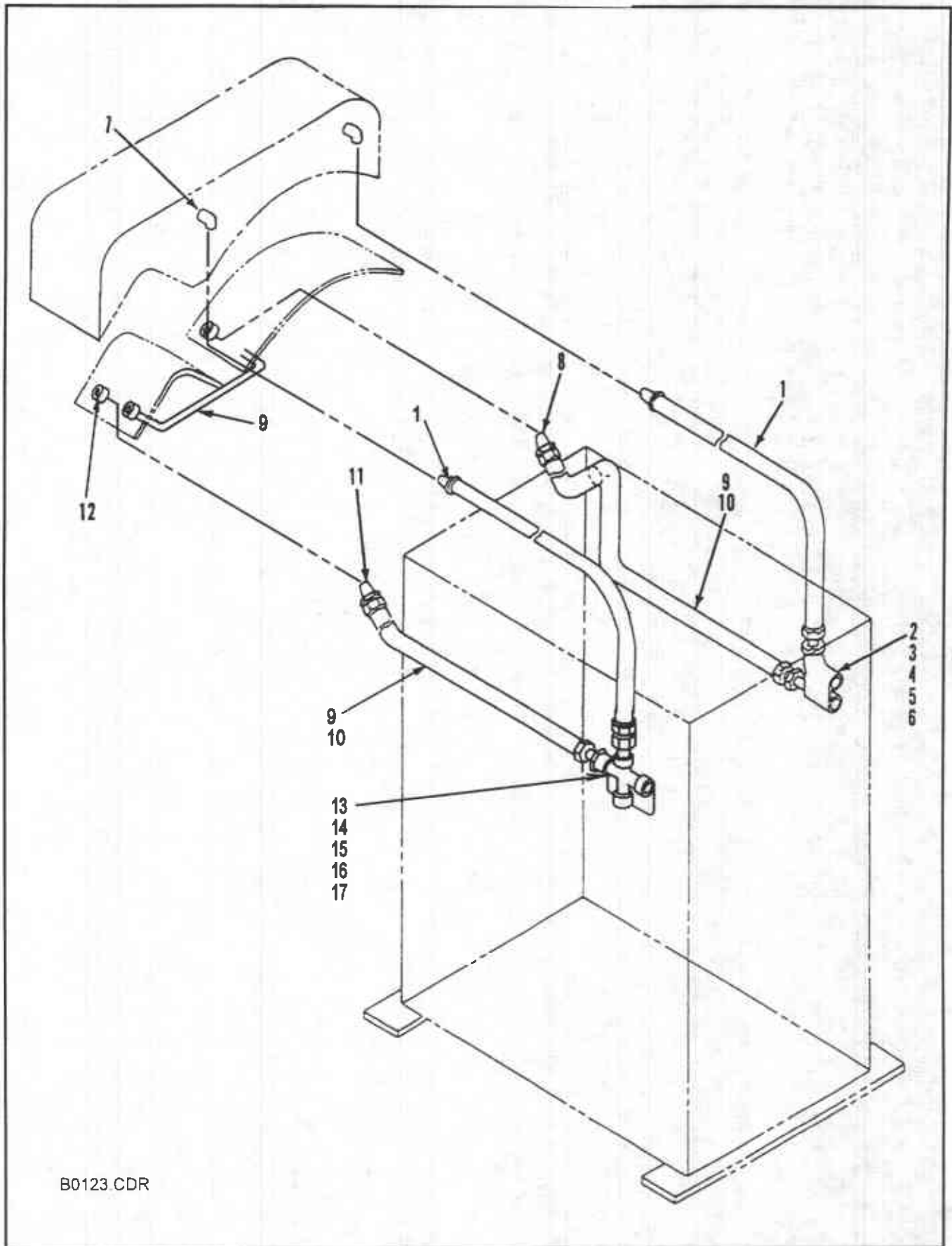
Figure 6-16. Steam System
