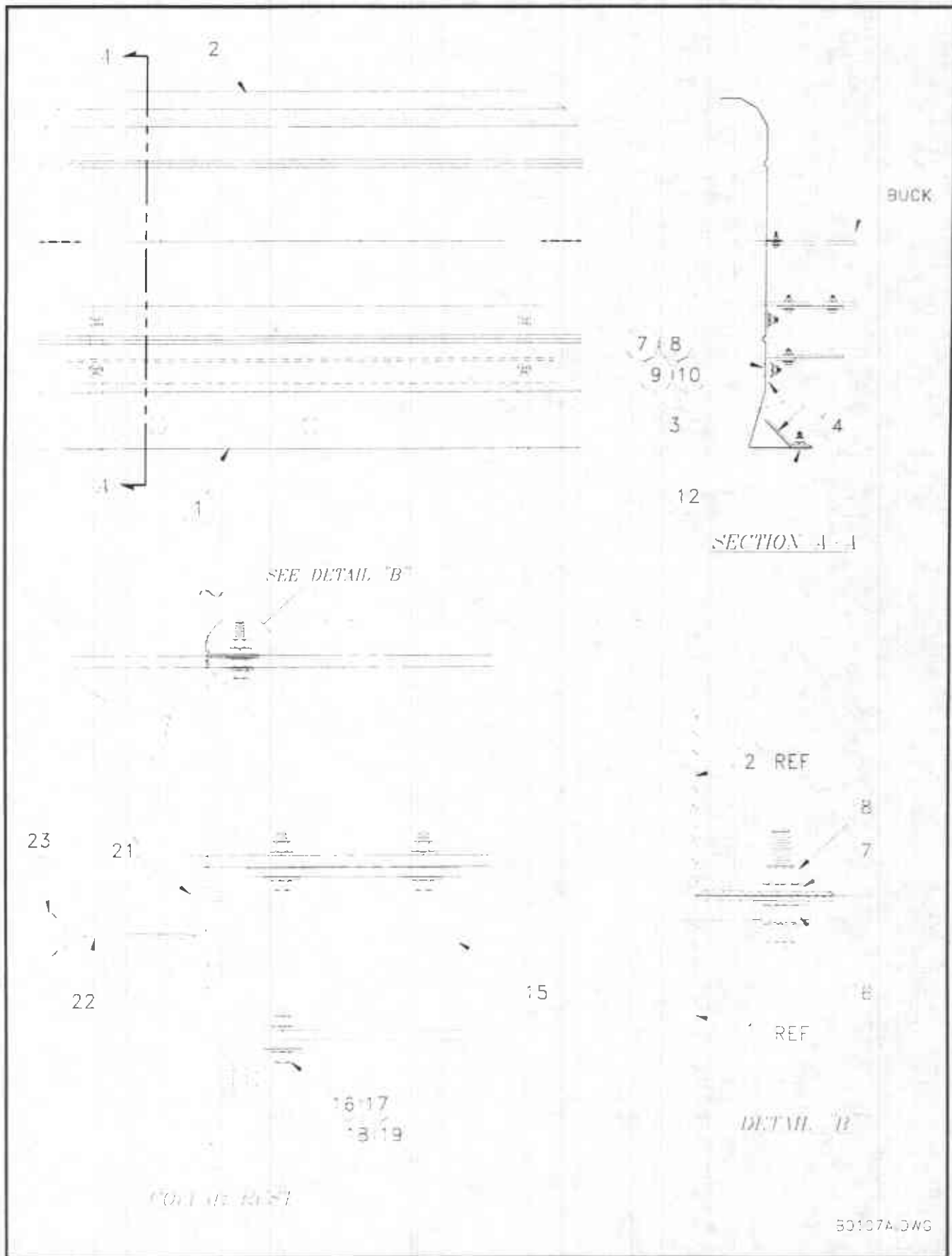
Figure 6-25. Table Mounting
