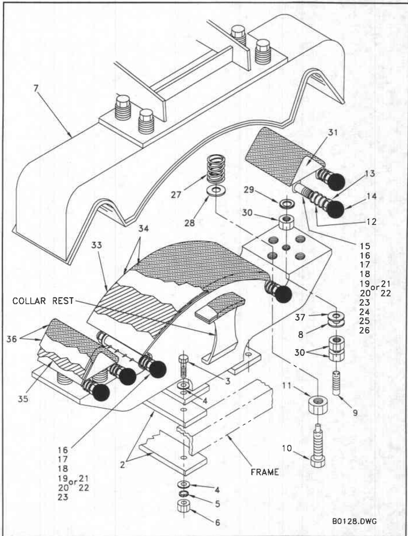
Figure 6-22. Buck Mounting
