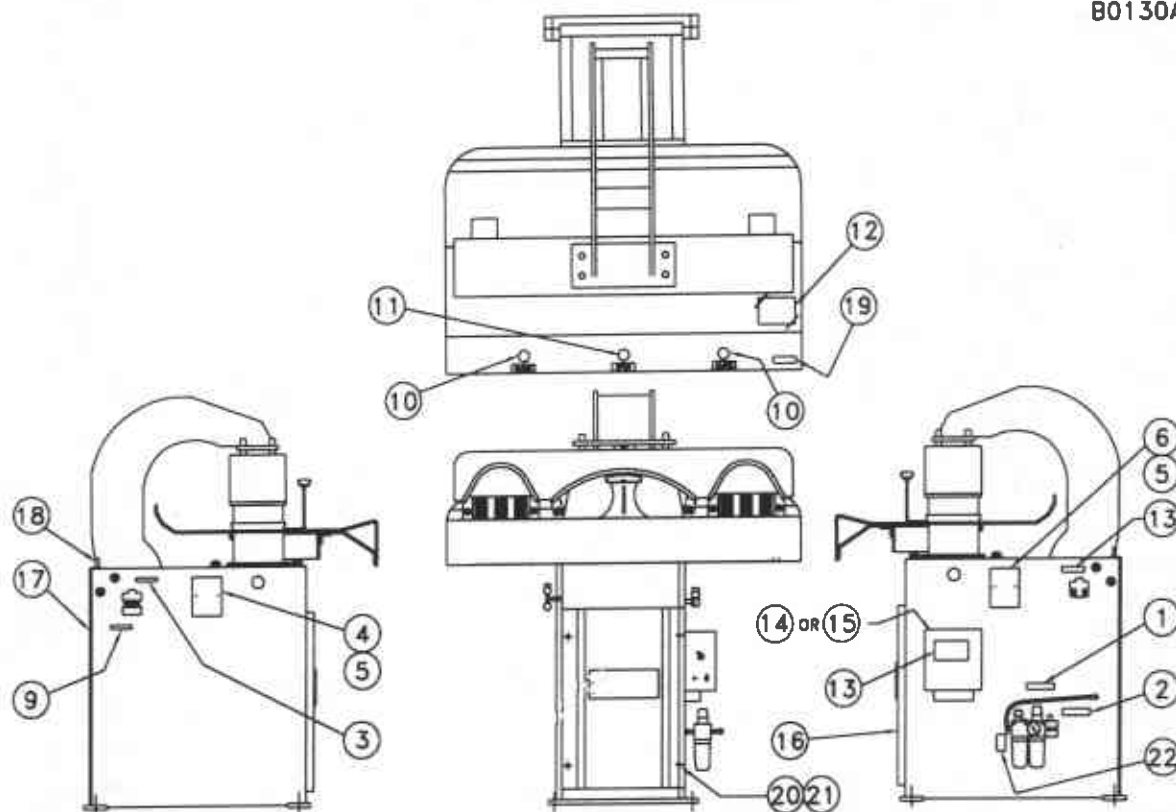
Figure 6-27. Labels
