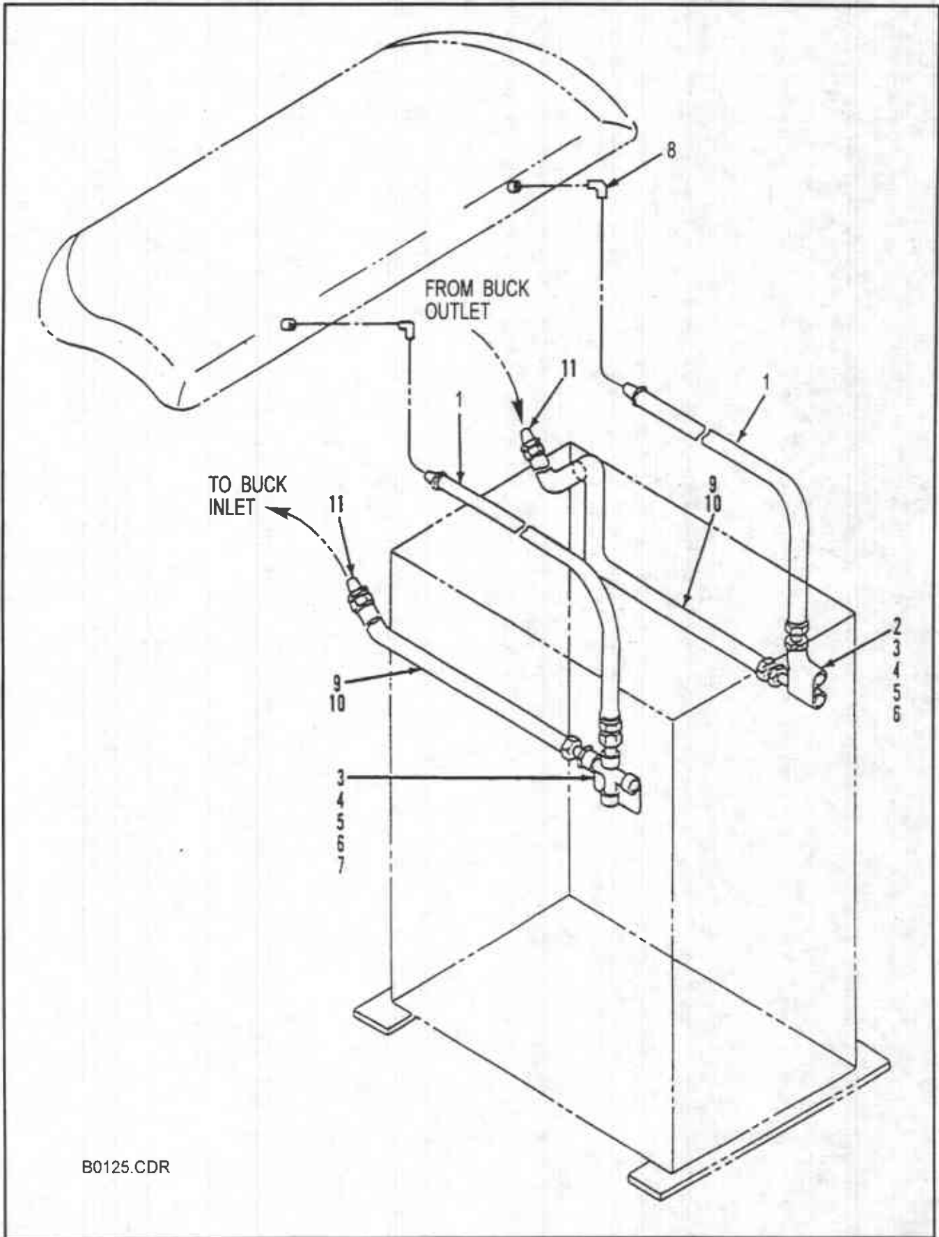
Figure 6-17. Steam System
