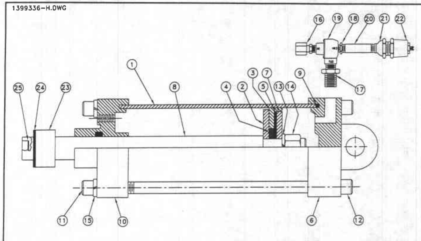
Figure 6-4. Air Cylinder Assembly - 6" Bore
