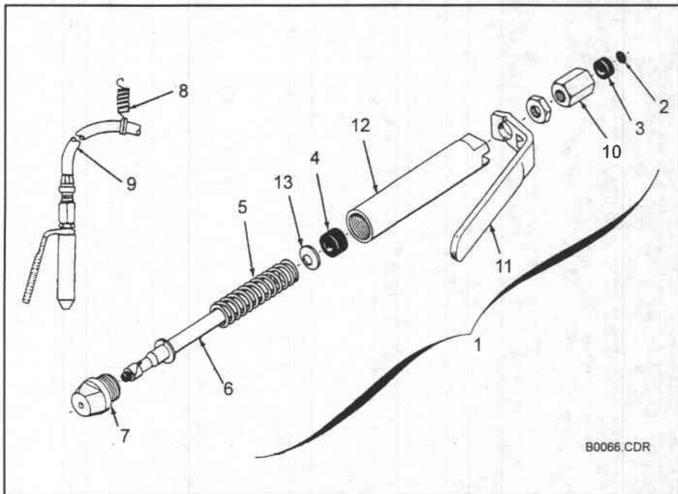
Figure 6-19. Water Gun Assembly
