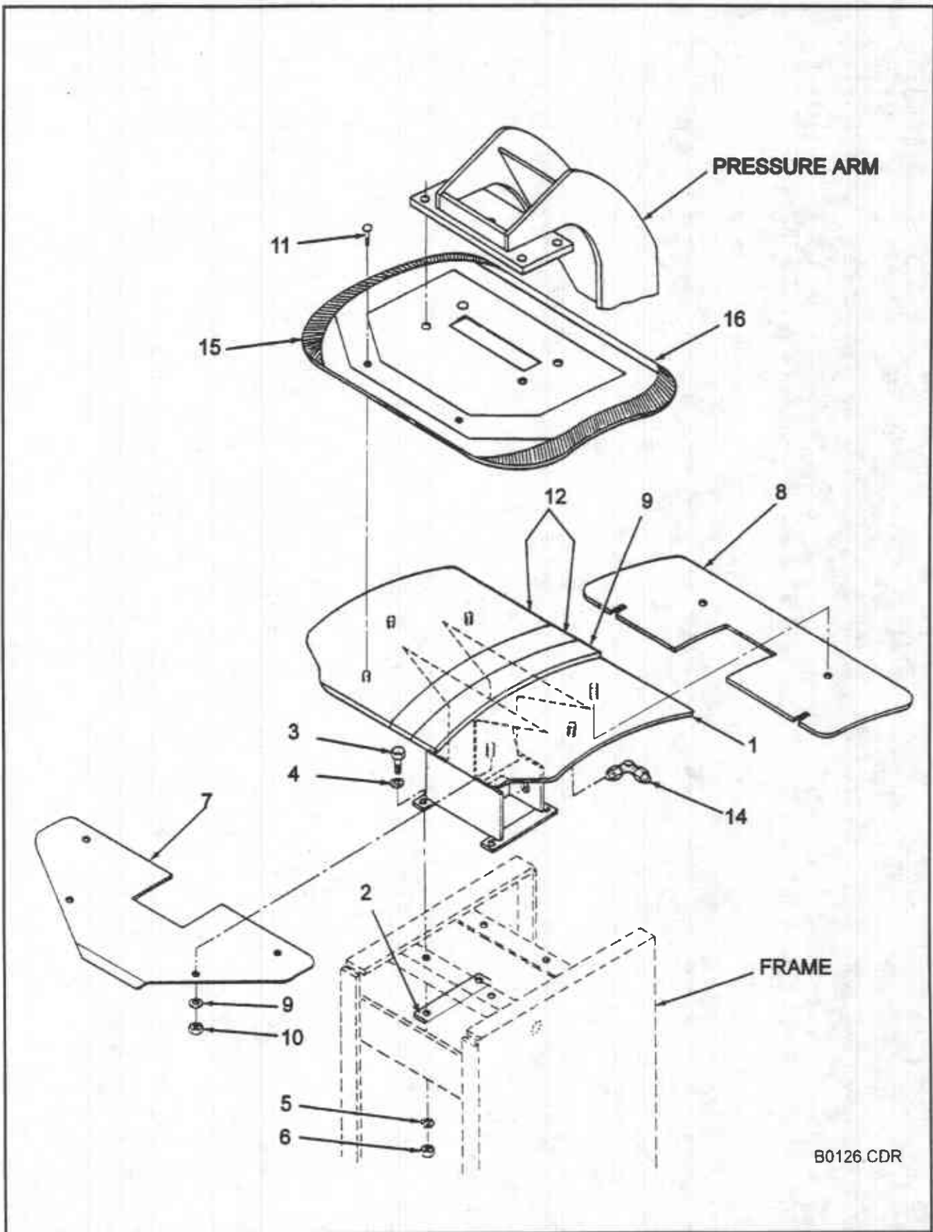
Figure 6-24. Buck Mounting
