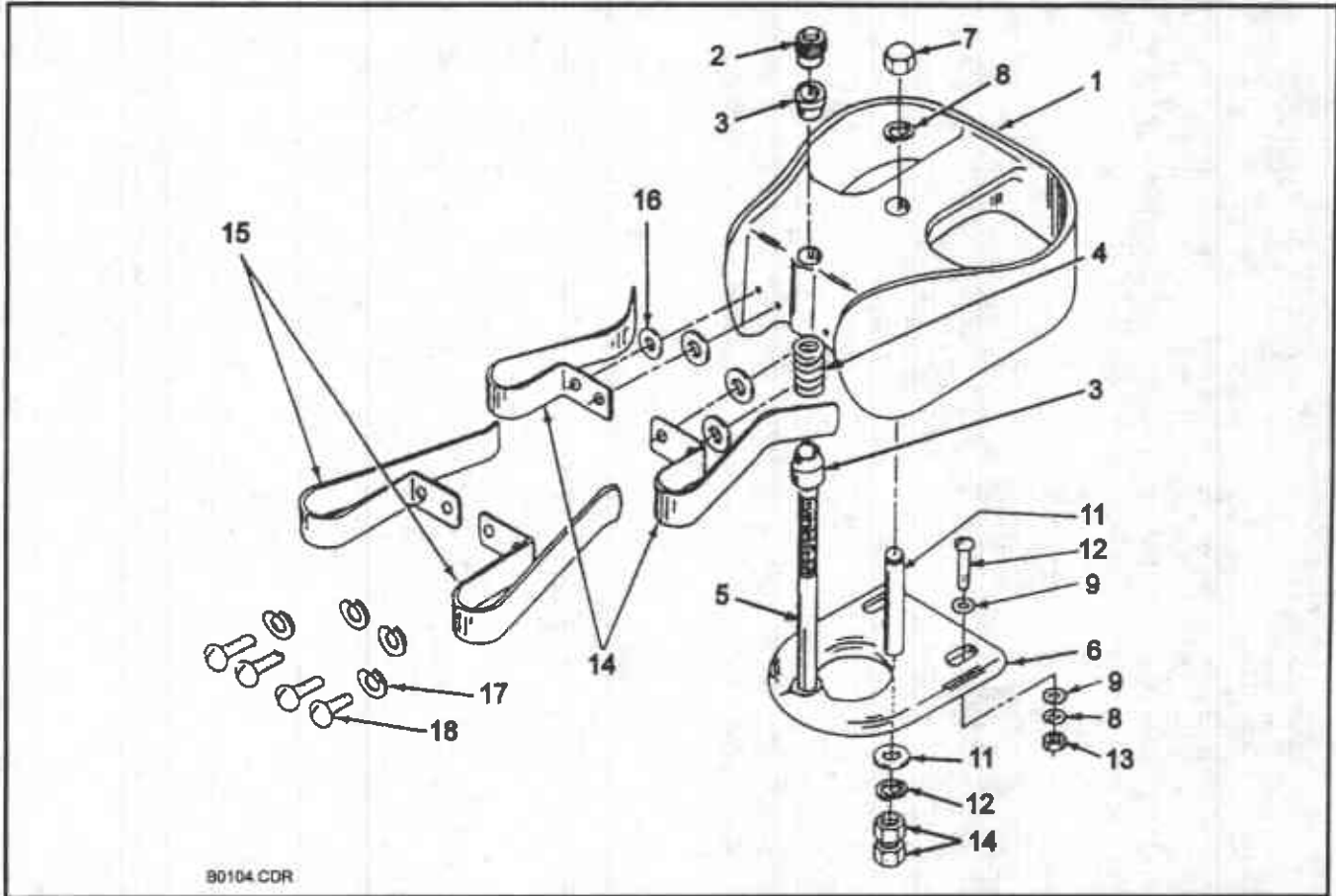
Figure 6-26. Yoke Block Assembly
